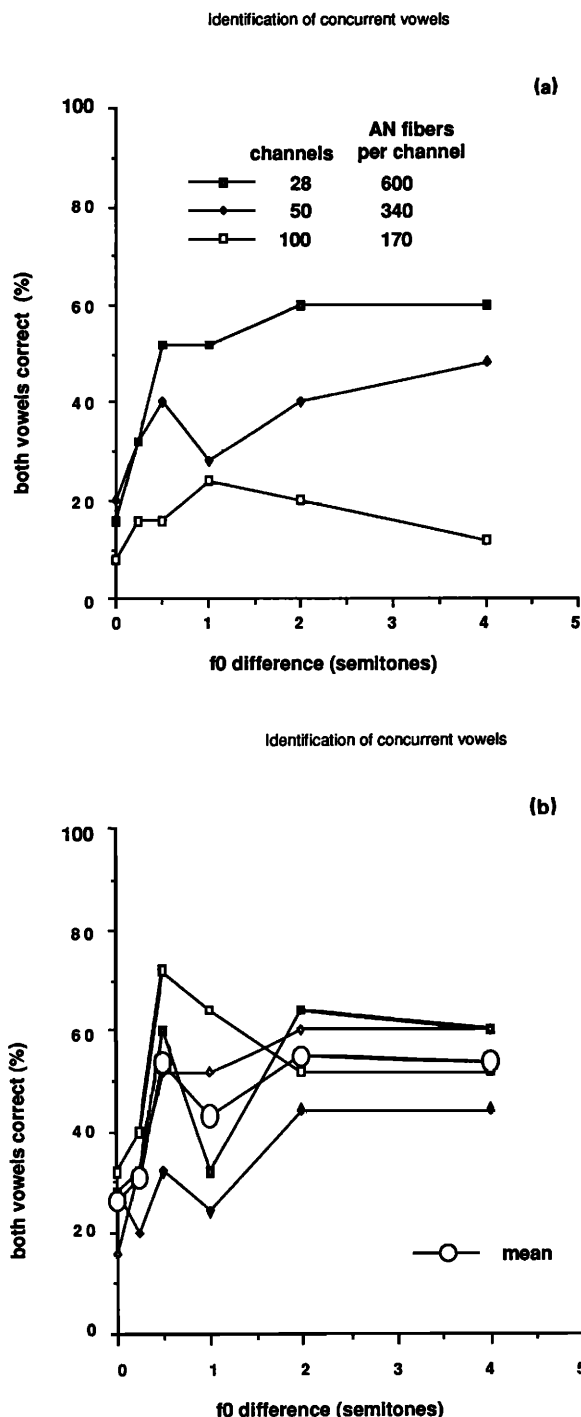
FIG. 15. (a) Performance of a stochastic version of the model (see text) compared for 100 channels with 170 fibers per channel, 50 channels with 340 fibers, and 28 channels with 600 fibers based on a single run for each. (b) Results for four runs of a 28 channel model with 600 fibers.
