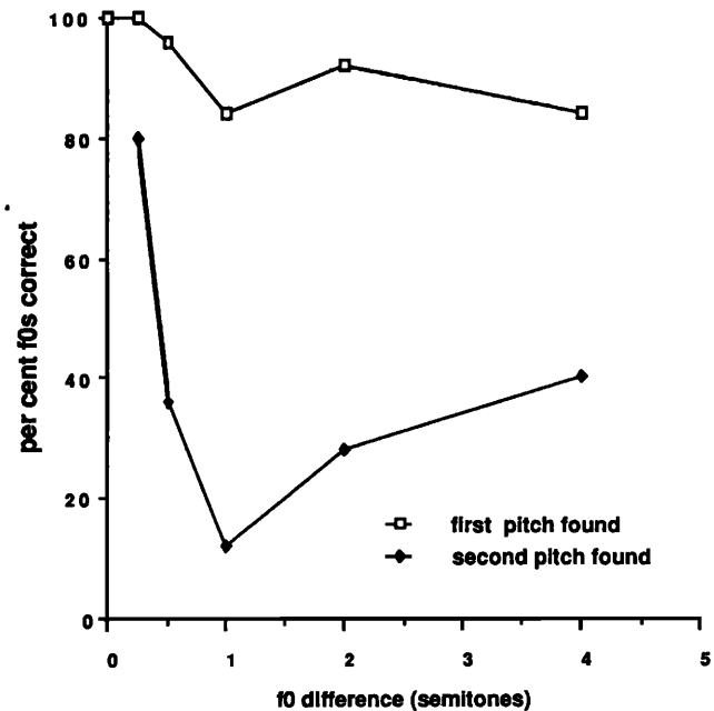
FIG. 11. Percentage correct estimation of the vowel fundamental frequency. The value for the second vowel is based only on those cases where the first vowel fundamental was estimated correctly.
