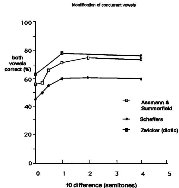
FIG. 1. Listeners' ability to correctly identify both vowels of a pair of simultaneous presented vowels as a function of the separation of the f_0 of the two vowels. Results taken from Scheffers (1983a), Zwicker (1984), and Assmann and Summerfield (1990).
