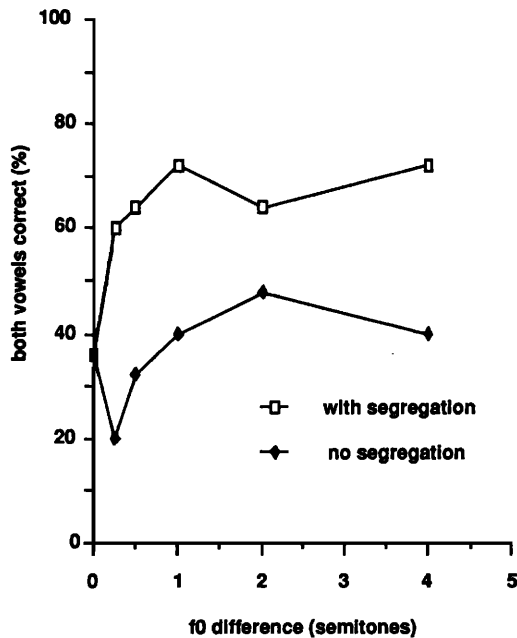
FIG. 10. Response of the model to the same stimuli as Fig. 9(a) except that the model was forced to respond without using any pitch information (i.e., rule 1 was set to judge only one pitch present for all stimuli). Results from Fig. 9(a) are included for comparison purposes.
