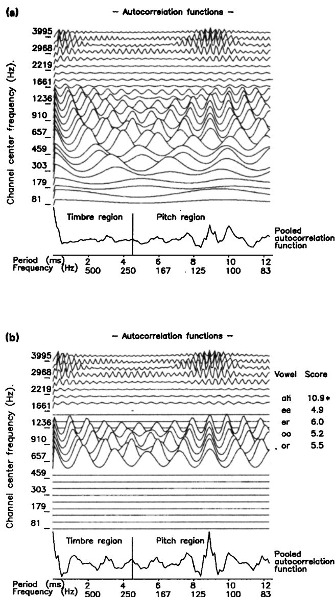
FIG. 7. (a) ACFs and pooled ACF for a stimulus consisting of two vowels ("er" and "ah") where both vowels are synthesised with two different f_0 (100 and 112 Hz, respectively). The first pitch is correctly judged to be 112 Hz using the highest peak in the pooled ACF. Forty nine channels showed a pitch peak at 112 Hz. (b) As in (a) but all channels which do not show a peak at 112 Hz have been set to zero. The inset values show the results of the matching algorithm using the new pooled ACF. The starred value shows the best matching vowel which is "ah." (c) As in (a) but all channels which do show a peak at 112 Hz have been set to zero; i.e. (c) is the complement of (b). The best match to the new pooled ACF is seen to be "er."
